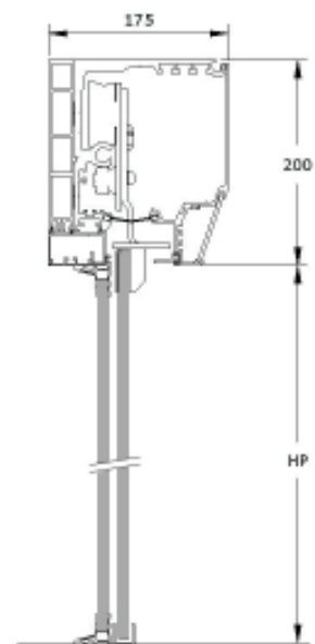
LUMINA with DIVA reinforced casing
