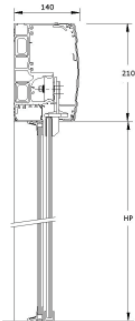
LUMINA with DIVA L Reinforced casing
