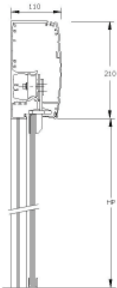
LUMINA with standard DIVA L casing
